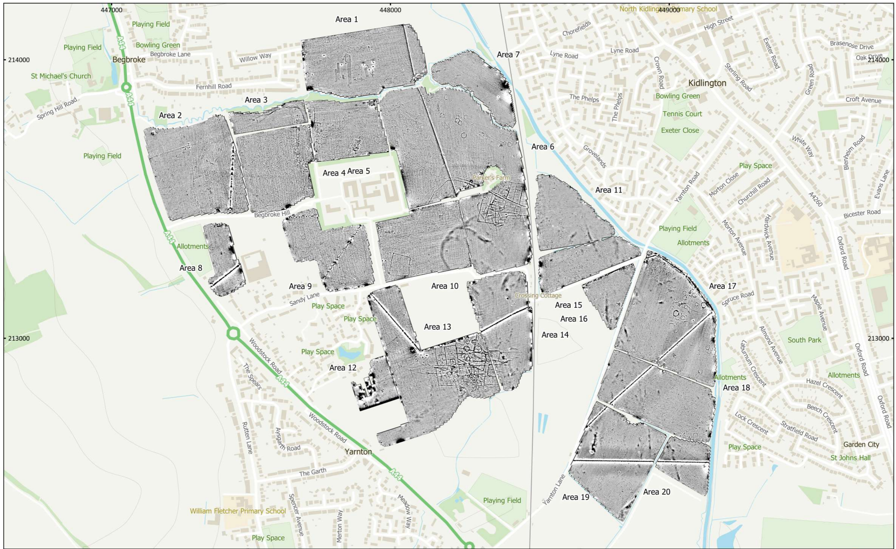
MSSP1306 - Begbroke, Oxfordshire Figure 9 - Magnetic Gradient 1:8,000 @ A3 Copyright Magnitude Surveys Ltd 2022 Contains satellite imagery © 2022 Bing Satellite
