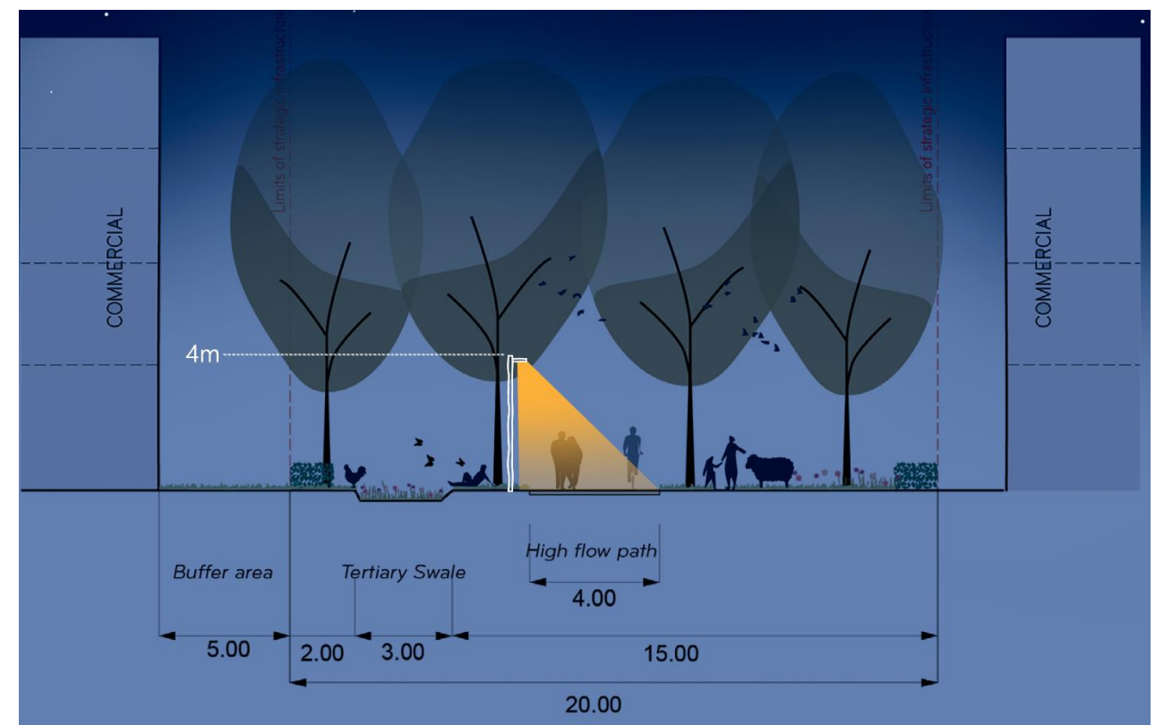
Figure 5.6 – Lighting strategy for a typical high flow shared surface path
